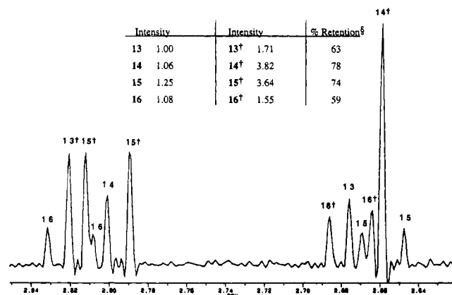
Figure 2. ^3\text{H}\{^1\text{H},^2\text{H}\} -NMR spectra (acetone- d_6 ) at 320 MHz of malate (7.5 mCi) derived from ( R )-malonate 9 . The FIDs were accumulated and processed as in Figure 1 (except total acquisition time was 2.7 h and GB = 0.7 and LB = -0.8 for processing). Inset: Relative intensities of malate species derived from ( R )-[1- ^{13}\text{C} , 2- ^3\text{H} ]malonate. § Percent retention values for individual isotopomers.
