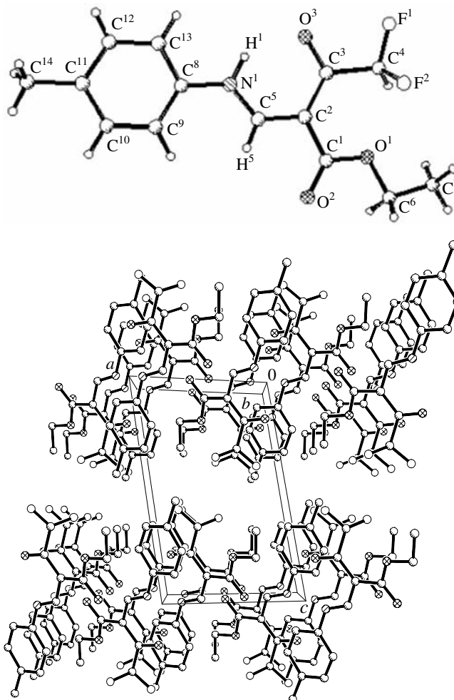
Fig. 1. Crystalline structure of ethyl 4,4-difluoro-2-(4-methylphenylaminomethylidene)-3-oxobutanoate ( VIIa ) according to the X-ray diffraction data.
