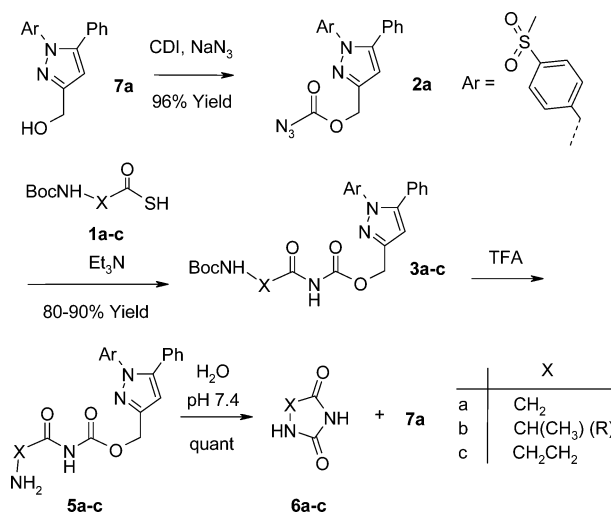
Scheme 2. Imide Ligation and Rearrangement Using Model Thioacids 1a–c
