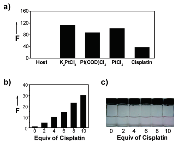
Figure 4. (a) Fluorescence intensities of 1 (5 \mu M) in the presence of 10.0 equiv of different platinum complexes at 25 °C (at 562 nm). (b) Fluorescence intensity changes of 1 (5 \mu M) upon addition of different amounts of cisplatin in H 2 O (DMSO 1% v/v) (at 562 nm). (c) Color change of 1 (5 \mu M) upon addition of different amounts of cisplatin in H 2 O (DMSO 1% v/v).
