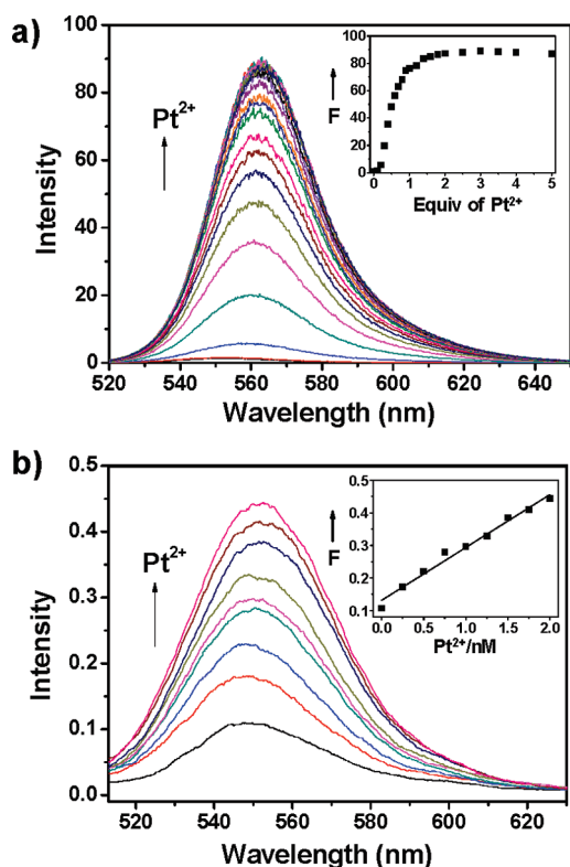
Figure 1. Fluorescence intensity changes of 1 upon additions of \text{Pt}^{2+} in \text{H}_2\text{O} (DMSO 1% v/v). Each spectrum is observed after 30 min of each \text{Pt}^{2+} addition at 25^\circ\text{C} with excitation at 500 nm. (a) 1 ( 5\ \mu\text{M} ). Inset: plot of fluorescence intensities at 562 nm depending on the equivalents of \text{Pt}^{2+} . (b) 1 ( 0.5\ \mu\text{M} ) upon additions of \text{Pt}^{2+} (by 125 nM). Inset: plot of fluorescence intensities at 553 nm depending on the concentration of \text{Pt}^{2+} .
