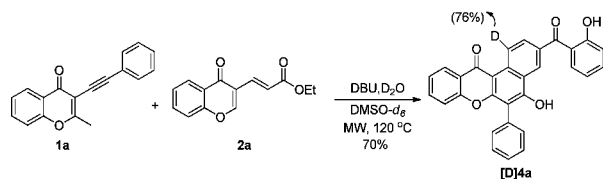
Scheme 3. Deuterium Labeling Experiment in the Reaction of 1a with 2a
