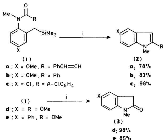
Scheme 1. Reagents and conditions: i, LDA, THF, -20°C, 20 min.
