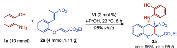
Scheme 3. The Cascade Reaction Was Performed on a Gram Scale
