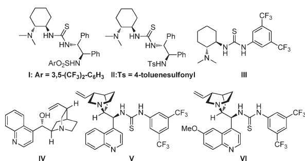
Figure 1. Screened organocatalysts.
