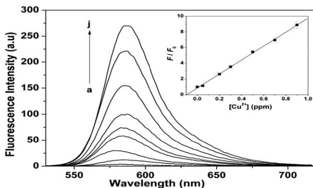
Fig. 1 Emission spectra of 1 (1.0 \mu\text{M} ) in the presence of various concentrations of \text{Cu}^{2+} in 20% (v/v) water–methanol solution (0.02 M HEPES, pH 6.0). [\text{Cu}^{2+}] : (a) 0 to (j) 6.0 \mu\text{M} . Inset: Linear fluorescence intensity ( F/F_0 ) of 1 (1.0 \mu\text{M} ) upon addition of \text{Cu}^{2+} (0–0.9 \mu\text{M} ). The response ( F ) is normalized to the emission of the free probe 1 ( F_0 ).
