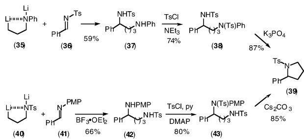
Scheme 3. Synthetic Manipulation Solely Based on Amino Groups
