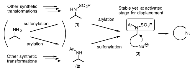
Scheme 1. Formulation of Synthetic Utility
