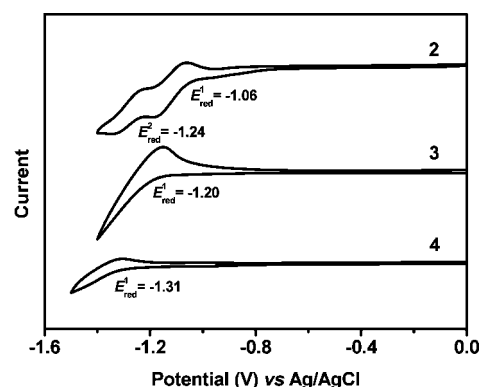
Figure 4. Cyclic voltammograms of 2–4 in hot chlorobenzene ( 70^\circ\text{C} ) under nitrogen atmosphere with 0.1 M \text{Bu}_4\text{NPF}_6 as supporting electrolyte, \text{AgCl}/\text{Ag} as reference electrode, Au disk as working electrode, Pt wire as counter electrode, and scan rate at 50 mV/s.
