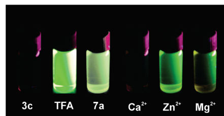
Figure 3. From left to right: compound 3c dissolved in \text{CH}_2\text{Cl}_2 ; compound 3c after the addition of trifluoroacetic acid; compound 7a , compound 3c after the addition of \text{Ca}^{+II} triflate; compound 3c after the addition of \text{Zn}^{+II} triflate; compound 3c after the addition of \text{Mg}^{+II} triflate; (irradiation at \lambda_{\text{exc}} = 354 \text{ nm} ).
