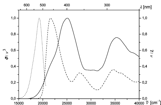
Figure 2. UV-vis and emission spectra of 3c and 3c-H + recorded in \text{CH}_2\text{Cl}_2 at 298 K. Absorption spectra of 3c (solid line) and 3c-H + (after protonation with TFA, dashed line); emission spectrum of 3c-H + (dotted line).
