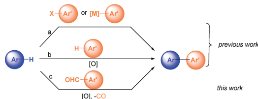
Scheme 1. Arene–Arene Coupling via C–H Activation
