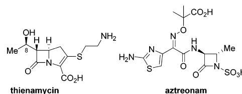
Figure 1. Representative \beta -lactam structures.
