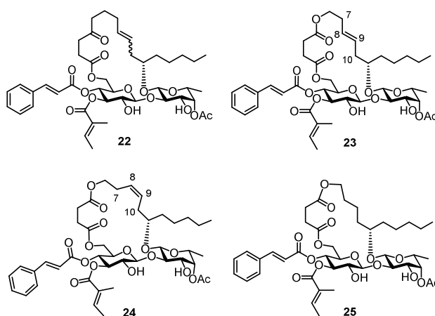
Figure 3. Structures of aglycone-modified ipomoeassin F analogues 22–25 .
