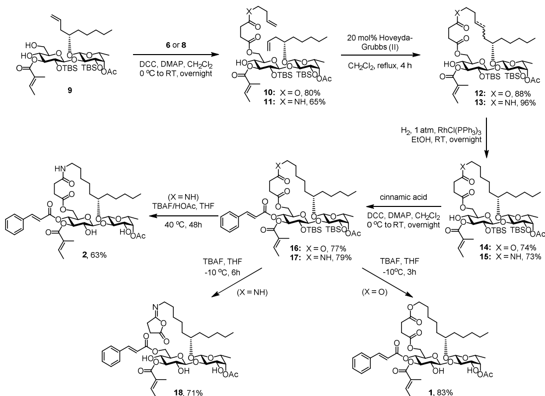
Scheme 2. Synthesis of Bioisosteric 5-Oxa/Aza Analogues (1 and 2) of Ipomoeassin F
