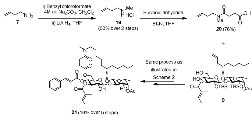
Scheme 3. Synthesis of Methylated 5-Aza Analogue ( 21 ) of Ipomoeassin F
