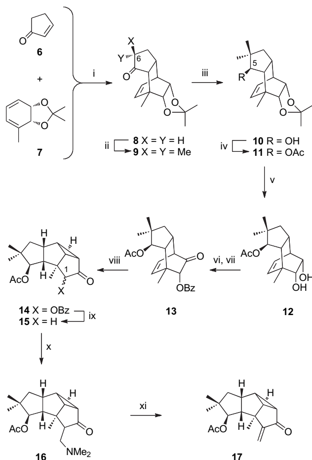
Scheme 1. Reagents and conditions: (i) see ref. 3b; (ii) LiHMDS (1.1 mol equiv), THF, –15→18→–15 °C, 1.25 h then MeI (1.2 mol equiv), 0.75 h then –15→18 °C (over 1.25 h) then repeat procedure; (iii) LiAlH 4 (1.5 mol equiv), Et 2 O, –30→18 °C, 6.5 h; (iv) Ac 2 O (3 mol equiv), DMAP (cat.), Et 3 N, 0→18 °C, 16 h; (v) H + -DOWEX-50, MeOH/H 2 O, reflux, 20 h; (vi) 4-AcNH-TEMPO (2.2 mol equiv), p -TsOH·H 2 O (2.2 mol equiv), CH 2 Cl 2 , 0→18 °C, 7 h; (vii) BzCl (2.5 mol equiv), DMAP (3.3 mol equiv), Et 3 N (excess), CH 2 Cl 2 , 0→18 °C, 16 h; (viii) acetophenone (1.4 mol equiv), acetone, photolysis, 18 °C, 3.5 h; (ix) SmI 2 (2.2 mol equiv), THF/MeOH, –78 °C, 0.16 h; (x) LiHMDS (1.2 mol equiv), THF, –78 °C, 1 h then Eschenmoser's salt (3 mol equiv), –78→18 °C, 16 h; (xi) MeI (12 mol equiv), Et 2 O/CH 2 Cl 2 , 18 °C, 16 h then Al 2 O 3 (basic), CH 2 Cl 2 , 18 °C, 0.5 h.
