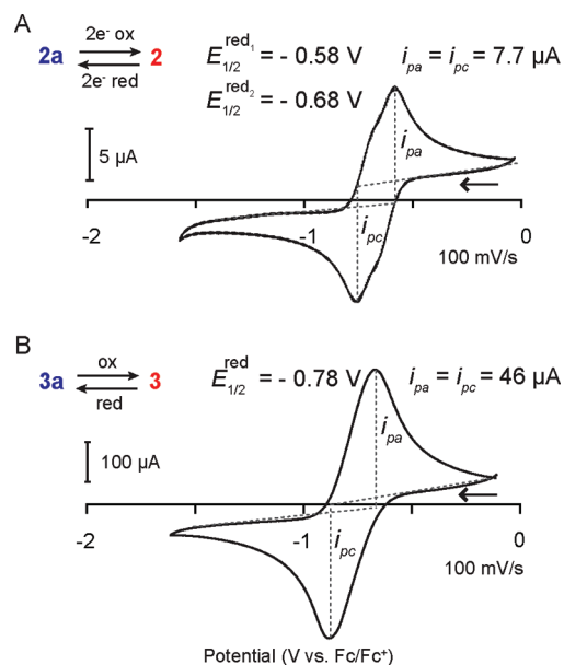
Figure 3. Cyclic voltammograms of 2 (a) and 3 (b) showing the reversible redox couple between the carbanion and the radical. Conditions: (a) 0.10 M LiClO 4 in DMF, Pt-button electrode, [ 2a ] \approx 1 \text{ mM} , 2a formed by deprotonation with LiOt-Bu in DMF; (b) 0.10 M ( n -Bu) 4 NPF 6 in MeCN, Pt-wire electrode with 3 dropcast from a chloroform solution.
