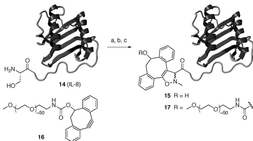
Scheme 2. One-pot N-terminal functionalization of IL-8 by SPANC: a) 1. \text{NaIO}_4 , \text{NH}_4\text{OAc} buffer, pH 6.9, room temperature, 1 h; 2. p\text{-MeOC}_6\text{H}_4\text{SH} , room temperature, 2 h; b) p\text{-MeOC}_6\text{H}_4\text{NH}_2 , \text{MeNHOH}\cdot\text{HCl} , room temperature, 20 min; c) cyclooctynol 2 or PEG-cyclooctyne 16 , room temperature, 20 h.
