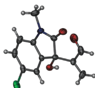
Figure 2. X-ray structure of 4f .
