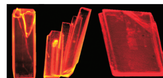
Figure 3. Photographs of solid-state fluorescent single crystals of the 4-aminoprop-3-enylidene indolones 8a (left), 8m (center), and 8n (right) ( \lambda_{\text{excitation}} = 460 nm).
