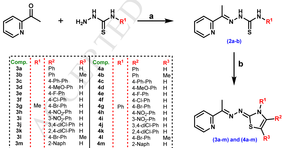
Scheme 2. Synthetic procedures for thiosemicarbazones ( 2a-b ) and 2-(pyridin-2-yl)-1,3-thiazoles ( 3a-m ; 4a-m ). Reagents and conditions: (a) 4-methyl-3-thiosemicarbazide or 4-phenyl-3-thiosemicarbazide, ethanol, acetic acid (5 drops), rt, 120 min; (b) halo-substituted acetophenones, 2-propanol, ultrasound irradiation, r.t., 60 min; R 3 = H for all compounds, except to ( 3b ), ( 3l ), ( 4b ) and ( 4l ) where R 3 = Me.
