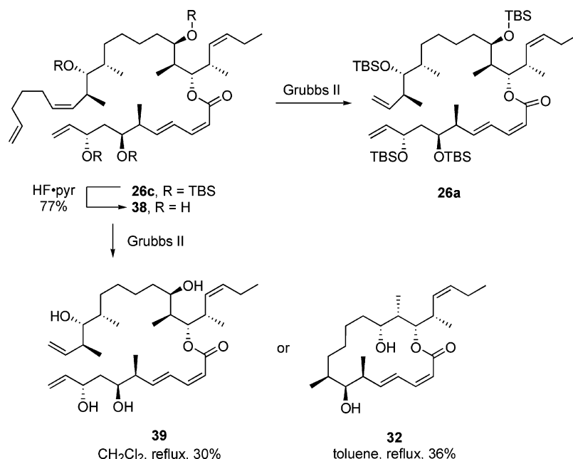
Scheme 10. Synthesis and RCM Reaction of 26d
