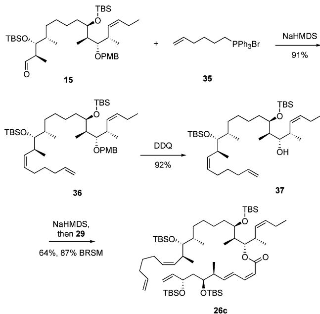
Scheme 8. Synthesis of RRCM Precursor 26c
