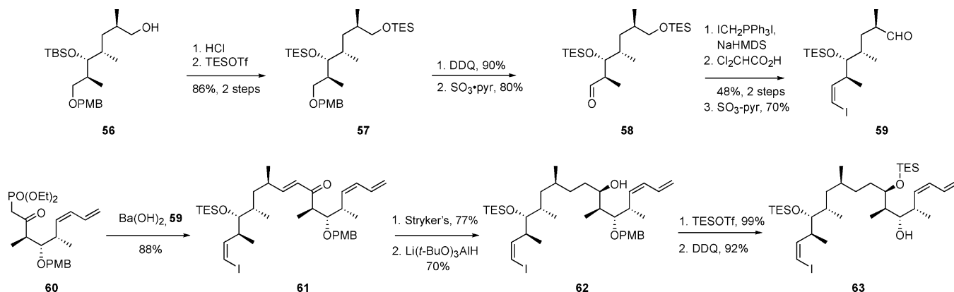
Scheme 13. NHK Route to Dictyostatin: Synthesis of the Top-Middle Fragment 63 , C10–C26
