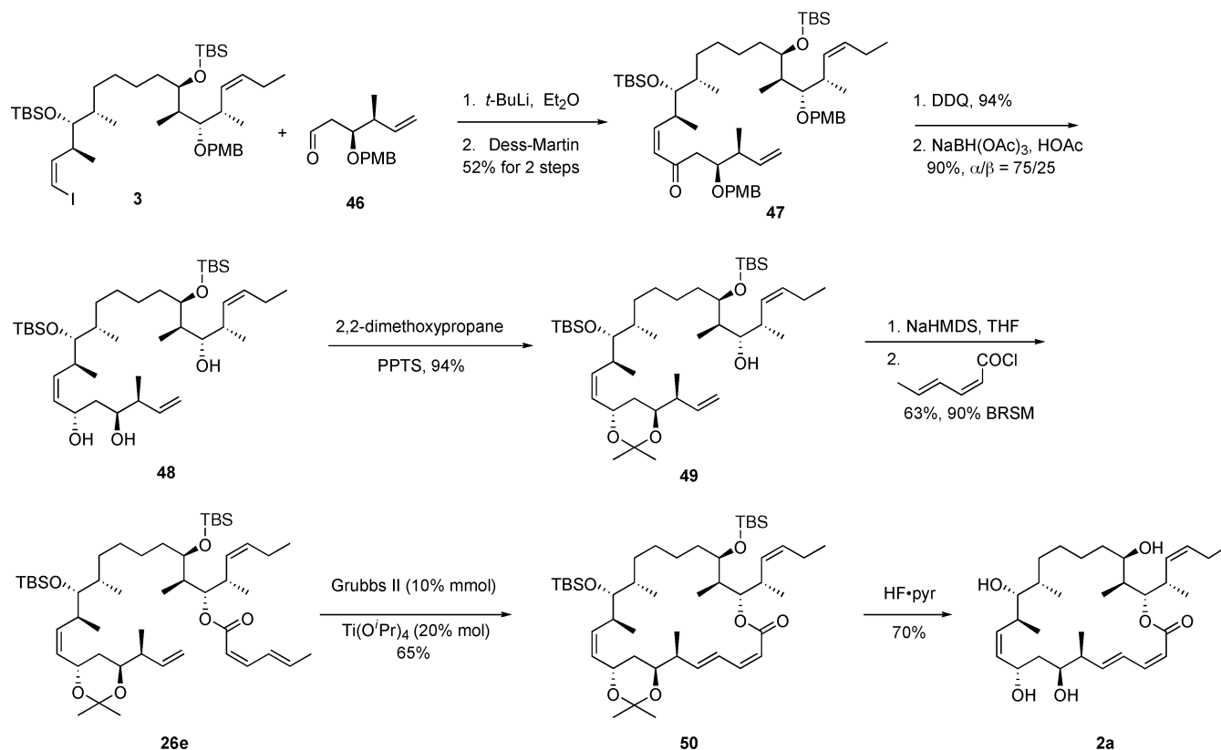
Scheme 11. Successful RCM Route to 2a
