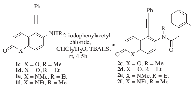
Scheme 1. Synthesis of precursors 2a–f .
