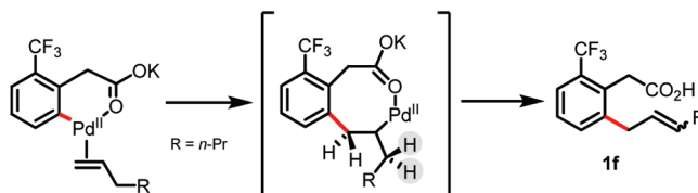
Scheme 6. Mechanistic Hypothesis to Explain the Preferential Formation of 1f , Rather than the Thermodynamically Favored Conjugated Product
