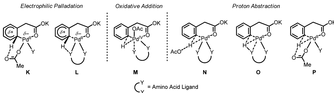
Scheme 12. Proposed Catalytic Cycle
