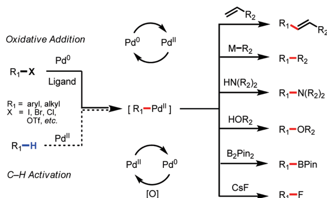
Scheme 1. Versatile Reactivity of [Pd(II)–R] Intermediates
