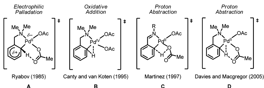
Scheme 8. Conceptually Relevant Proton Abstraction Mechanistic Proposals for Pd(0)/ArX Catalytic Systems
