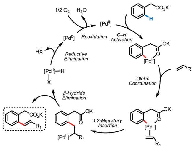
Scheme 12. Proposed Catalytic Cycle
