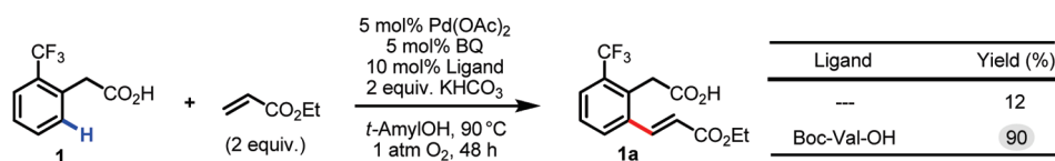
Scheme 3. Preliminary Results for Ligand-Promoted C–H Olefination of 1 45
