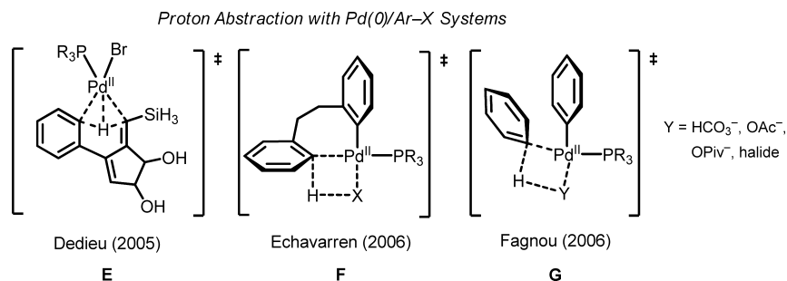
Scheme 8. Conceptually Relevant Proton Abstraction Mechanistic Proposals for Pd(0)/ArX Catalytic Systems
