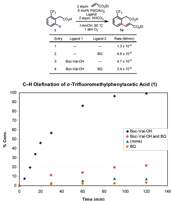
Figure 1. Initial rate studies of C–H olefination of o -trifluoromethylphenylacetic acid ( 1 ). BQ (5 mol %) and Boc-Val-OH (10 mol %). Each data point represents the average of three trials, with the exception of Boc-Val-OH data points from 60 to 120 min, which each represent a single trial. See Supporting Information for experimental details.
