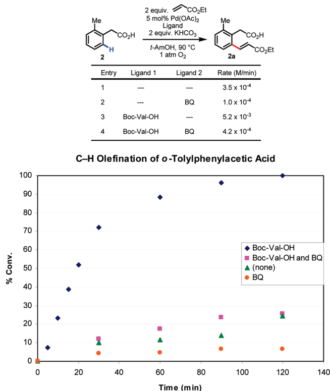
Figure 2. Kinetic studies of C–H olefination of o -tolylacetic acid ( 2 ). BQ (5 mol %) and Boc-Val-OH (10 mol %). Each data point represents the average of three trials, with the exception of the Boc-Val-OH trials from 60 to 120 min, which represent single trials. See Supporting Information for experimental details.
