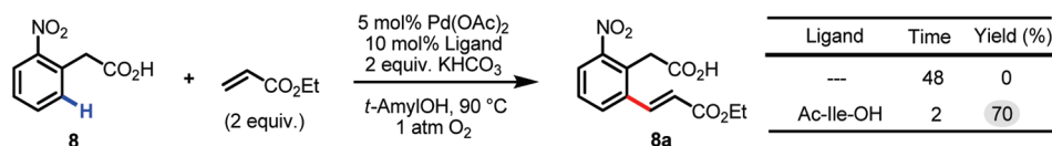
Scheme 9. Qualitative Evidence for a Change in the Mechanism of C–H Cleavage: C–H Activation of Highly Electron-Deficient Arenes in the Presence of Ac-Ile-OH
