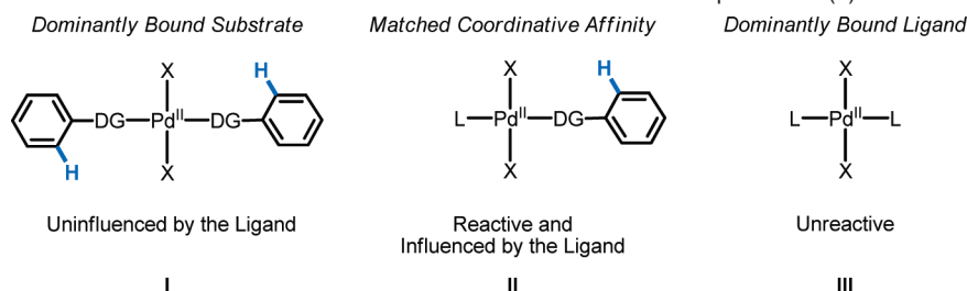
Scheme 2. Depiction of Three Scenarios for the Pretransition State Coordination Structures prior to Pd(II)-Mediated C–H Cleavage a
