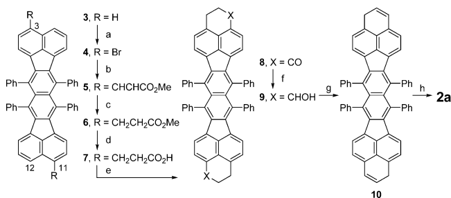
Scheme 2. Synthesis of 2a a
