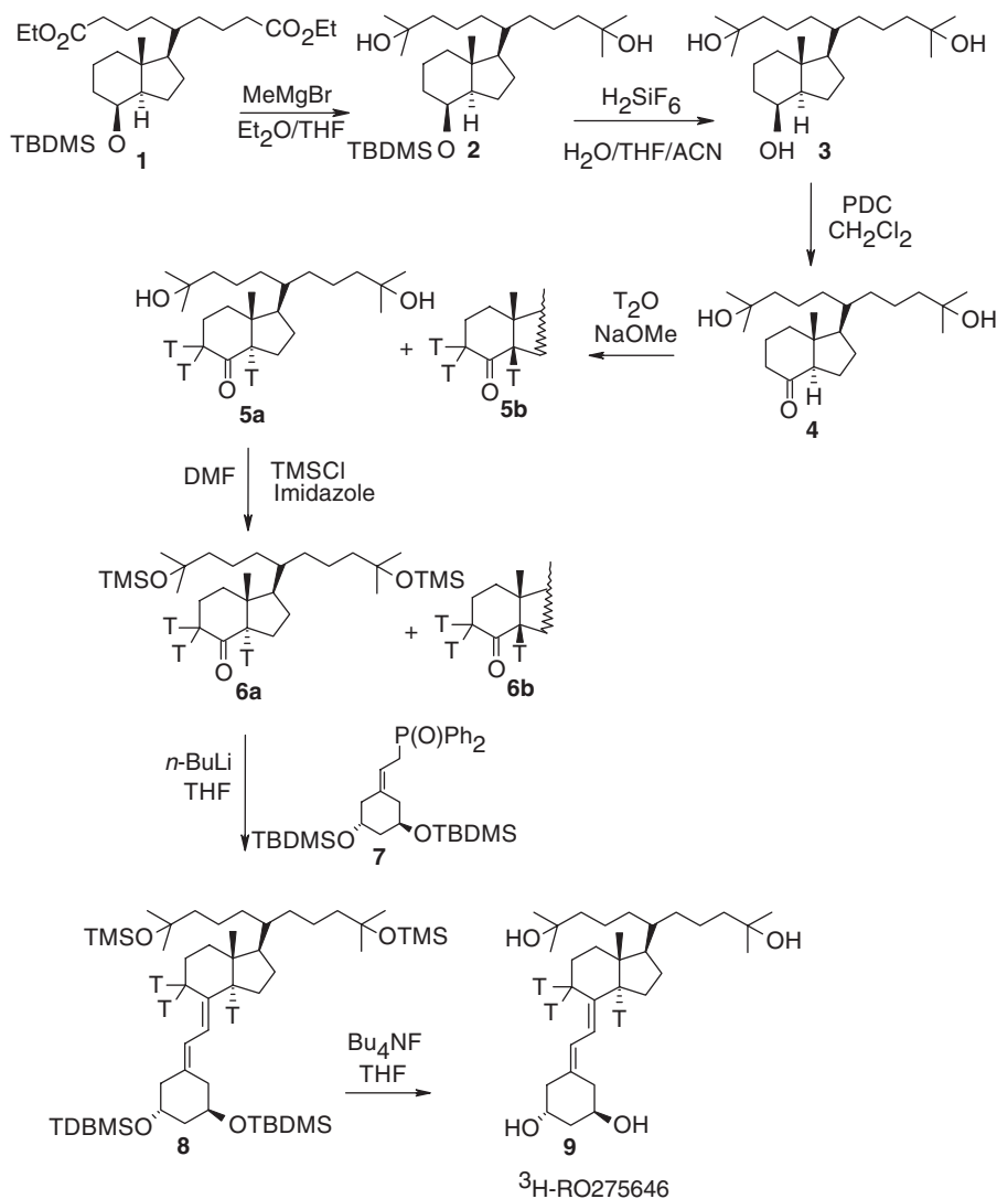
Scheme 2. Preparation of [ 3 H]-RO275646
