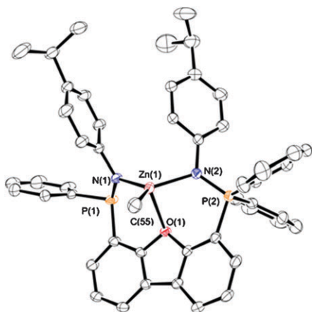
Fig. 1 X-Ray crystal structure of the cation of 2b , with ellipsoids shown at the 30% level. Hydrogen atoms, disordered atomic positions, and a phenyl group of P(1) have been omitted for clarity.
