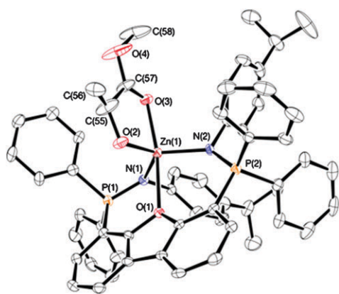
Fig. 2 X-Ray crystal structure of the cation of 3 , with ellipsoids drawn at the 30% probability level. Hydrogen atoms and disordered atomic positions have been omitted for clarity.
