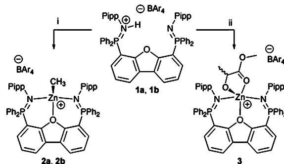
Scheme 1 Synthesis of cationic complexes 2a and 2b , and the cationic zinc–lactate complex 3 by reaction of (i) 1a (Ar = m -(CF 3 ) 2 -C 6 H 3 ) or 1b (Ar = C 6 H 5 ) with ZnMe 2 and (ii) 1a with EtZn(methyl-L-lactate).
