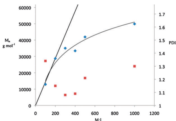
Fig. 3 Plot of observed M_n (◆) and PDI (■) as a function of the monomer to catalyst ratio. The straight line represents calculated M_n values ( M_n = [LA]_0 : [3] \times 144.13 ), while the curved line shows the general trend for experimental M_n values.
