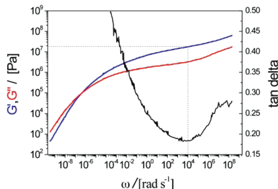
Figure 8. Master curve for the supramolecular network [ 1+2 ], with a reference temperature of 30^\circ C . The storage modulus profile is shown in blue, the loss modulus profile in red, and \tan \delta in black.
