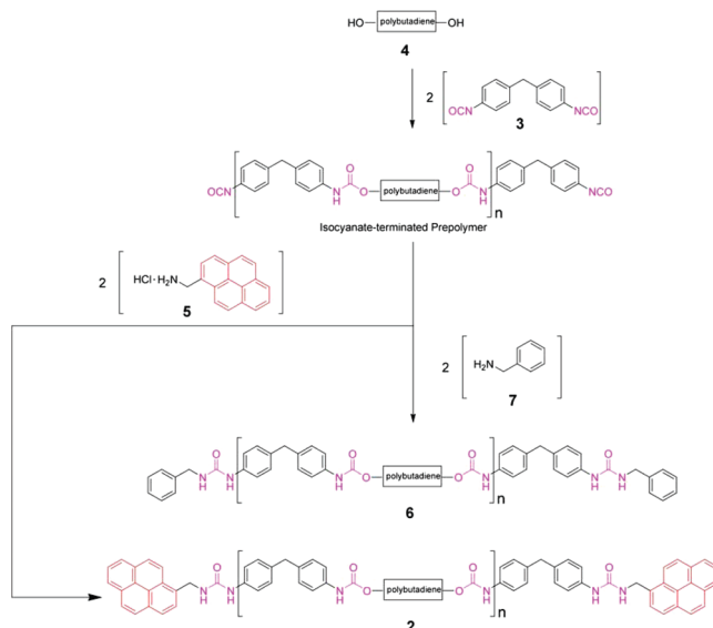
Scheme 1. Synthesis of Pyrenemethyl End-Capped Hydrogen-Bonding Polymer 2 and Benzyl End-Capped Polymer 6
