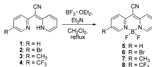
Scheme 1. Synthesis of Pyridomethene–BF 2 Complexes
