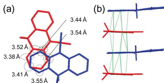
Figure 2. Crystal packing of 5 : (a) top view and (b) side view of 5 . Hydrogen atoms have been omitted for clarity. The dotted lines represent intermolecular C...C and C...N interactions.
