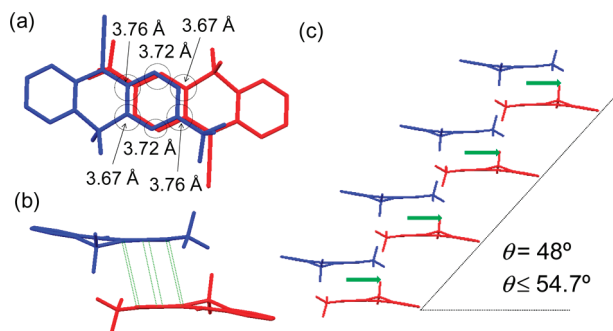
Figure 3. Crystal packing of 8 : (a) top view, (b) side view, and (c) stacking of 8 . Hydrogen atoms have been omitted for clarity. The dotted lines represent intermolecular C...C and C...N interactions. The green arrows indicate the transition dipole moment.
