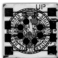
Figure 3. Picture of a transparent device containing a blend of 10c :PC 61 BM (25/75 wt %) lying on the seal of the Universität Würzburg.
