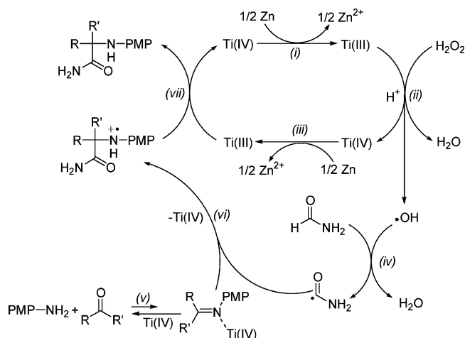
Scheme 2. Reaction Mechanism
