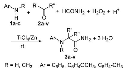
Scheme 1. Synthesis of Quaternary \alpha -Aminoamides Mediated by a \text{TiCl}_4/\text{Zn}/\text{H}_2\text{O}_2 System
