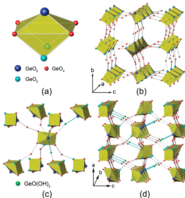
Figure 4. (a) \text{Ge}_7 cluster represented as a simplified polyhedron in which each vertex corresponds to a Ge atom. (b) Framework structure of PKU-10 by simplified polyhedra, showing the 13MR channels. (c) Each \text{Ge}_7 cluster surrounded by eight neighbors in a cubic environment. (d) Interaction between \text{GeO}(\text{OH})_3 tetrahedra and \text{Ge}_7 clusters by hydrogen bonds as indicated by blue dashed lines.
