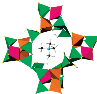
Figure 3. Location of the \text{TMA}^+ ion in the 13-ring channels of PKU-10.
