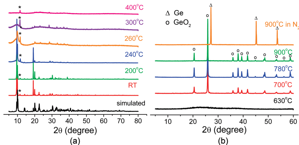
Figure 6. Powder X-ray diffraction patterns of PKU-10 calcined under atmospheres except the one marked with “in \text{N}_2 ”: (a) from the room temperature (RT) to 400 °C; (b) from 630 to 900 °C. The peaks marked by asterisks are from the impurity \text{Li}_3\text{HGe}_7\text{O}_{16} .
