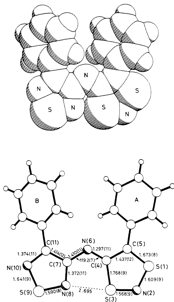
Figure 2. Space-filling and skeletal representations of the molecular structure of (7) showing selected bond lengths, angle and contact distance.
