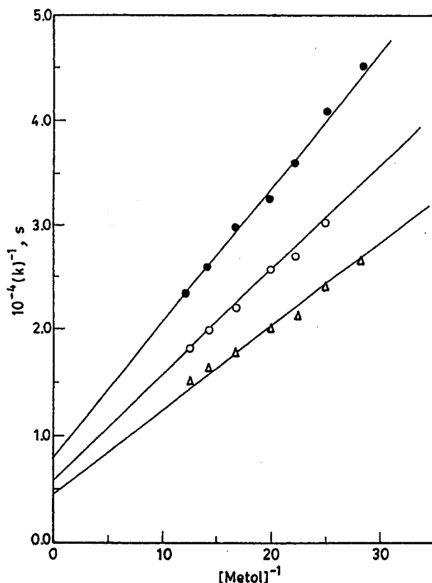
Figure 2. Metol concentration dependence. [\text{Tl}^{III}] = 4 \times 10^{-3} \text{ mol dm}^{-3} ; [H^+] = 0.5 \text{ mol dm}^{-3} ; •, 40^\circ \text{C} ; ○, 45^\circ \text{C} ; △, 50^\circ \text{C}
