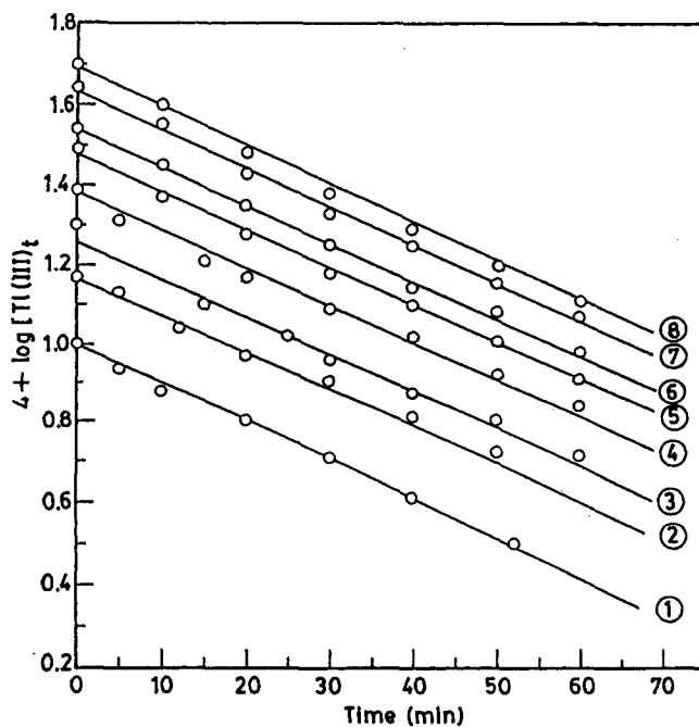
Figure 1. Pseudo-first-order plots. [\text{metol}] = 5 \times 10^{-2}\text{ mol dm}^{-3} ; [\text{H}^+] = 0.5\text{ mol dm}^{-3} ; temperature = 45^\circ\text{C} ; [\text{Ti}^{\text{III}}] ( \text{mol dm}^{-3} ) = ① 1.0 \times 10^{-3} ; ② 1.5 \times 10^{-3} ; ③ 2.0 \times 10^{-3} ; ④ 2.5 \times 10^{-3} ; ⑤ 3.0 \times 10^{-3} ; ⑥ 3.5 \times 10^{-3} ; ⑦ 4.5 \times 10^{-3} ; ⑧ 5.0 \times 10^{-3} .
