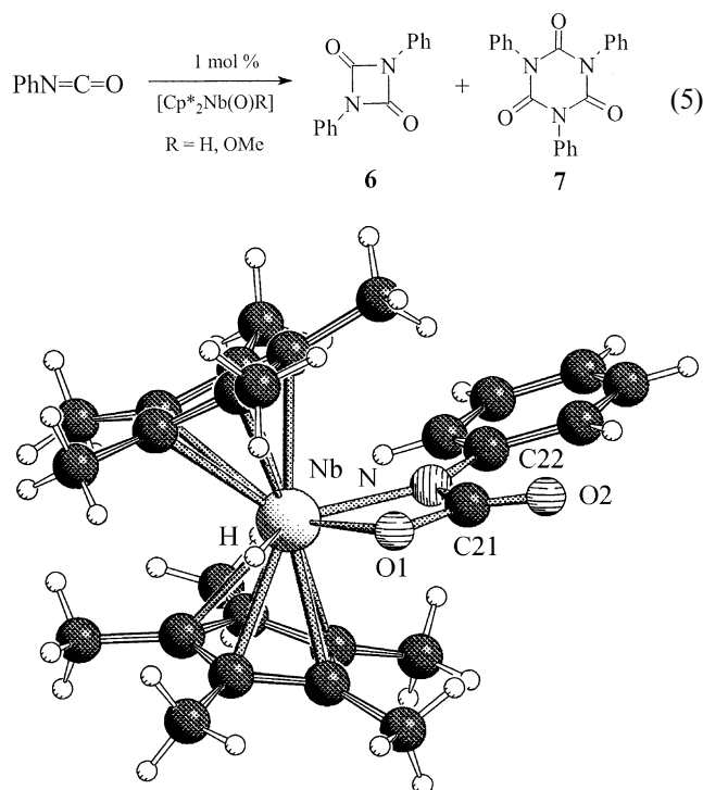
Fig. 3. Molecular structure of [\text{Cp}^*_2\text{NbH}\{\text{OC}(\text{O})\text{NPh}\}] ( 5 ).
