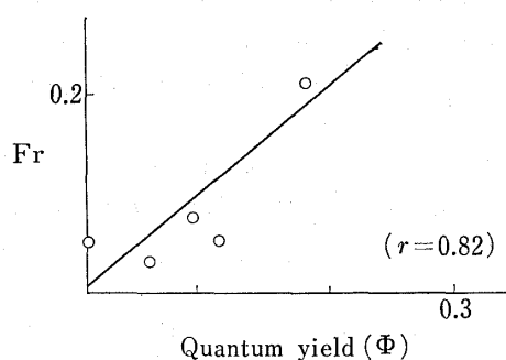
Fig. 1. Correlation ( r ) between Quantum Yields ( \Phi ) for the Products (17, 26, 27, 28, 34) derived from 1-Substituted Starting Materials and SOMO-ED of the 1-Methylindole Radical Cation (Fr)
