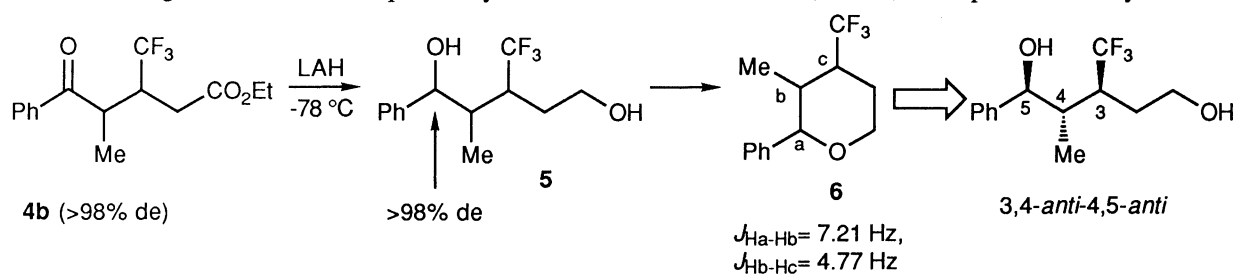
Scheme 2.
