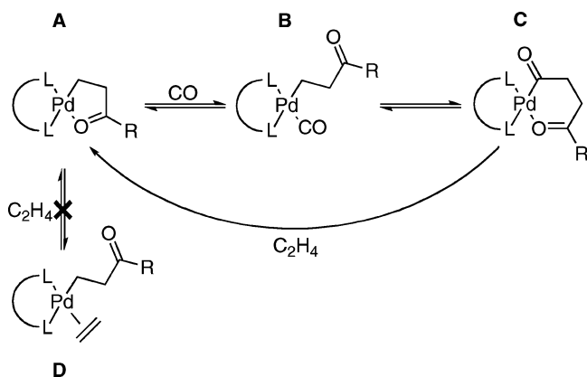
Scheme 1. General Catalytic Cycle for Ethene/Carbon Monoxide Copolymerization 1,4
