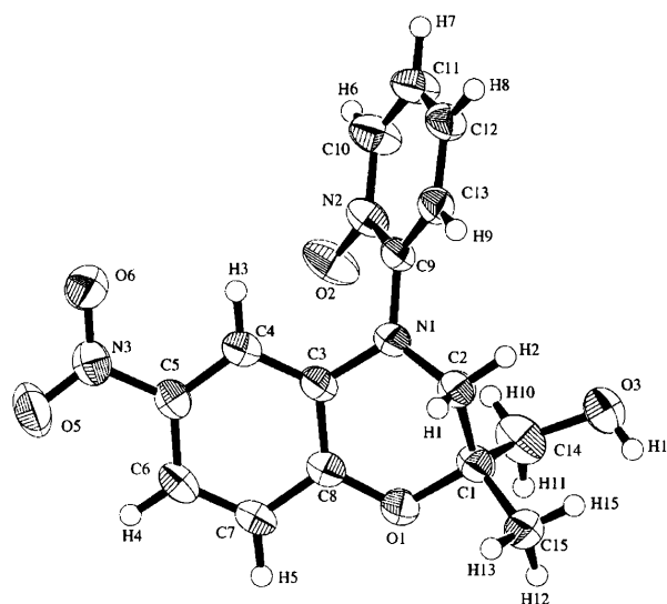
Fig. 1. X-Ray Structure of Compound 5
