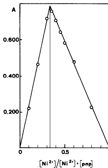
Fig. 1. Job's diagram for the system \text{Ni}(\text{H}_2\text{O})_6(\text{ClO}_4)_2 + \text{pnp} in \text{Me}_2\text{CO} . A = absorbance at 454 nm.
