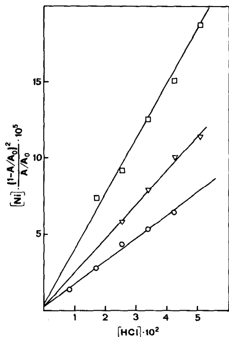
Fig. 2. Plot of [\text{Ni}] A_0 (1 - A/A_0)^2 / A vs. [\text{HCl}] for the system \text{Ni}(\text{pnp})\text{Cl}_2 + \text{H}_2\text{O} + \text{HCl} in n\text{-BuOH} . [\text{H}_2\text{O}] : \circ 2.22 M; \triangle 2.61 M; \square 3.11 M.
