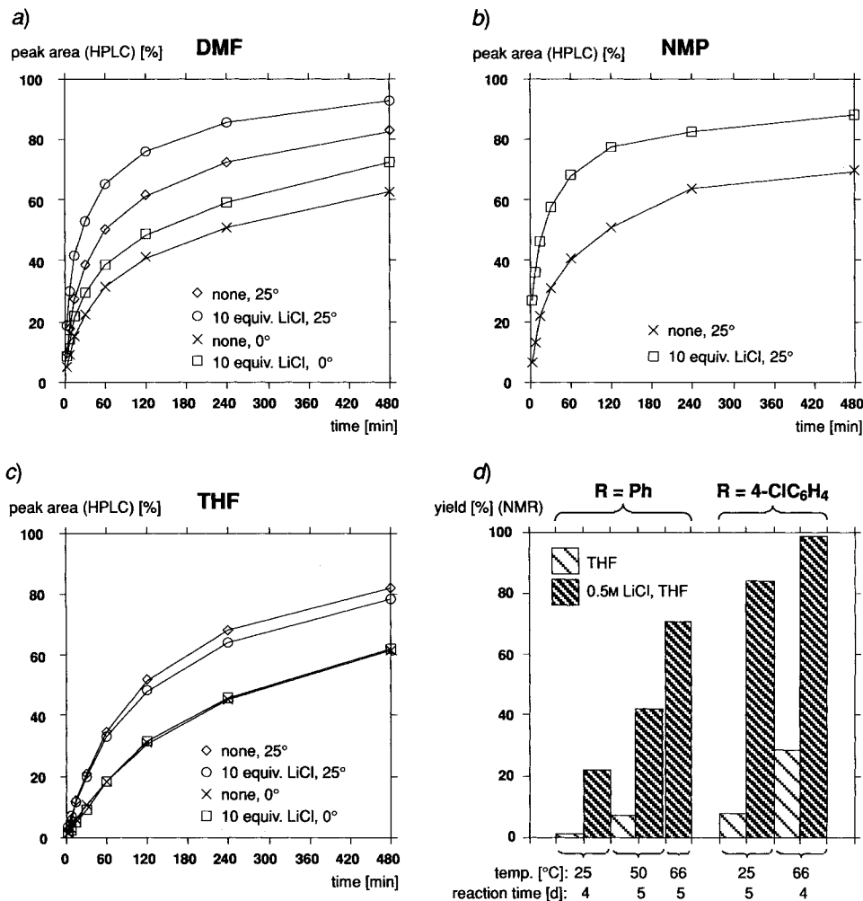
Figure. Coupling of phenylalanine derivatives (Z-Phe-OR) with \text{HCl} \cdot \text{H-Ala-O}(t\text{-Bu}) ( 11 ) using three different solvents and three different 'active' esters. a)–c) Kinetics of the coupling of Z-Phe-ONp ( 13 ) with 11 in different solvents (a): DMF; b): NMP; c): THF). d): Coupling yields using different phenylalanine derivatives in THF/LiCl and varying the reaction temperature and time (no detailed description of the experiments which led to the construction of diagram d) are given in the Exper. Part ; it was not checked whether epimerisation or side-product formation occurred in these experiments).
