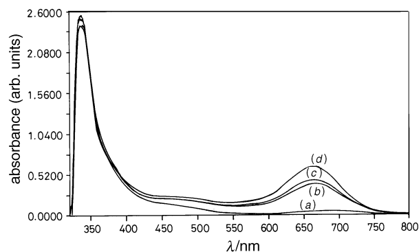
Fig. 5 Visible spectra for compound 3 in acetone (0.08 g l –1 ): (a) freshly prepared solution, and consecutive runs after (b) 1, (c) 2 and (d) 3 h, respectively
