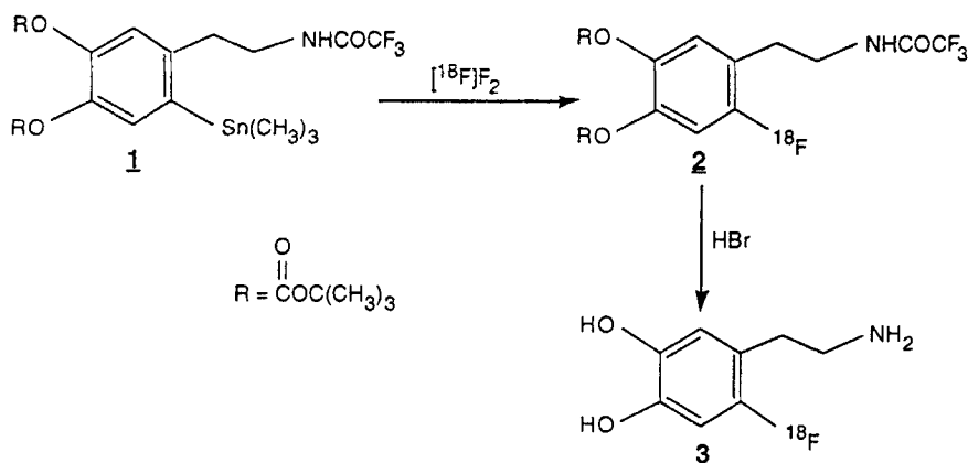
Scheme 1. Synthesis of 6- [^{18}\text{F}] fluorodopamines ( 3 ).
