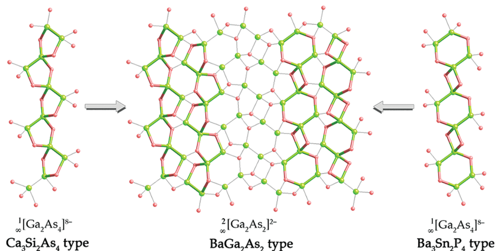
Figure 2. Schematic representation of the relationship between the \frac{2}{\infty}[\text{Ga}_2\text{As}_2]^{2-} layers in the structure of \text{BaGa}_2\text{As}_2 and the hypothetical \frac{1}{\infty}[\text{Ga}_2\text{As}_4]^{8-} chains, isosteric to \frac{1}{\infty}[\text{Si}_2\text{As}_4]^{6-} and \frac{1}{\infty}[\text{Sn}_2\text{P}_4]^{6-} known for the \text{Ca}_3\text{Si}_2\text{As}_4 (left) and the \text{Ba}_3\text{Sn}_2\text{P}_4 structure type (right), respectively. Color code as in Figure 1. Ba atoms are not shown for clarity. See the text for further details.
