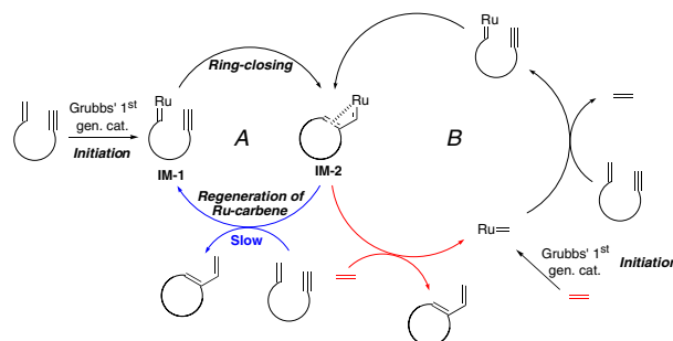
Fig. 1. Catalytic cycle of ring-closing enyne metathesis of terminal alkynes and the acceleration effect of ethylene. 6,9
