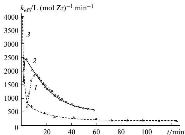
Fig. 5. Kinetic curves of propene bulk polymerization with the use of the 9 —TIBA—MAO catalytic system: Al(TIBA) : Zr = 1700 ( 1 ), 700 ( 2 ), and 220 ( 3 ). The polymerization temperature was 50 °C. For the polymerization conditions, see Table 5.
