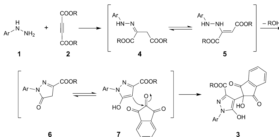
Scheme 2. A Plausible Mechanism for the Formation of 3
