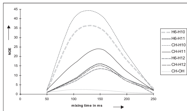
Fig. 6 Build-up curves of the seven most intense intraproton tr-NOE cross-peaks. (a) CH-OH; (b) H6-H12; (c) CH-H12; (d) H6-H11; (e) CH-H11; (f) H6-H10; (g) CH-H10. The parabolic behaviour is observed for all the peaks for N -dodecyl-2-(hydroxyiminomethyl)pyridinium bromide.
