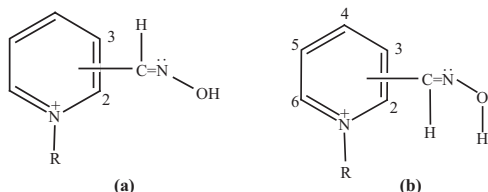
Fig. 1 (a) N -Alkyl pyridinium aldoxime bromides, showing the structure of anti forms, R is an alkyl group having general formula C_nH_{2n+1} where n varies from 2 to 16, -CH=NOH group present at 2, 3 or 4 positions of the pyridinium ring; (b) structure of syn forms.
