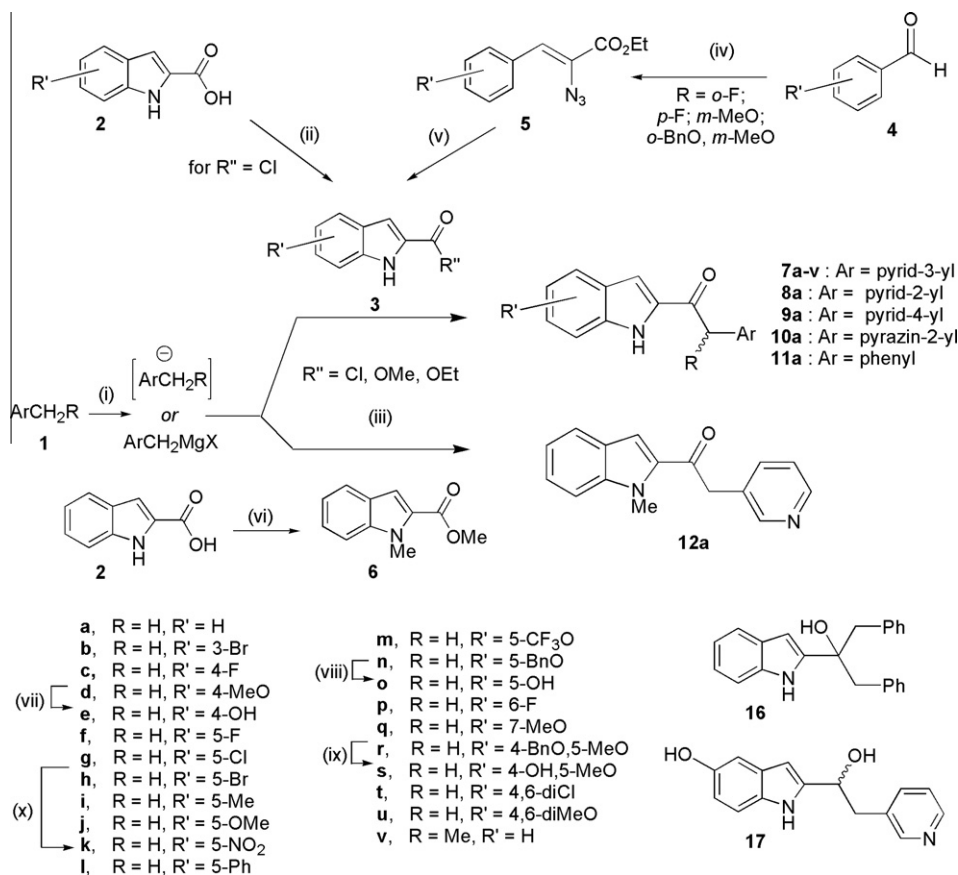
Scheme 1. General synthetic scheme for indol-2-yl ethanones. Reagents and conditions: (i) LDA, THF/hexanes, -78-0^\circ\text{C} , 1 h; (ii) \text{SOCl}_2 , \Delta , 15 min; (iii) THF/hexanes, 0^\circ\text{C} to rt, 16–24 h; (iv) \text{N}_3\text{CH}_2\text{CO}_2\text{Et} , NaOEt, EtOH, -10-4^\circ\text{C} , 1.5–20 h; (v) hexane, 200^\circ\text{C} ( \mu\text{W} ), 5 min; (vi) MeI, \text{K}_2\text{CO}_3 , DMF, 80^\circ\text{C} , 16 h to 5 days; (vii) \text{AlCl}_3 , \text{CH}_2\text{Cl}_2 , 0^\circ\text{C} to rt, 24 h; (viii) \text{HCO}_2\text{NH}_4 , Pd black, MeOH, rt, 1 h; (ix) \text{H}_2 (1 atm), 3% Pd/C, EtOH, rt, 45 min; (x) \text{PhB}(\text{OH})_2 , \text{Pd}(\text{PPh}_3)_4 , \text{K}_2\text{CO}_3 , EtOH/toluene 1:1, \Delta , 20 h.
