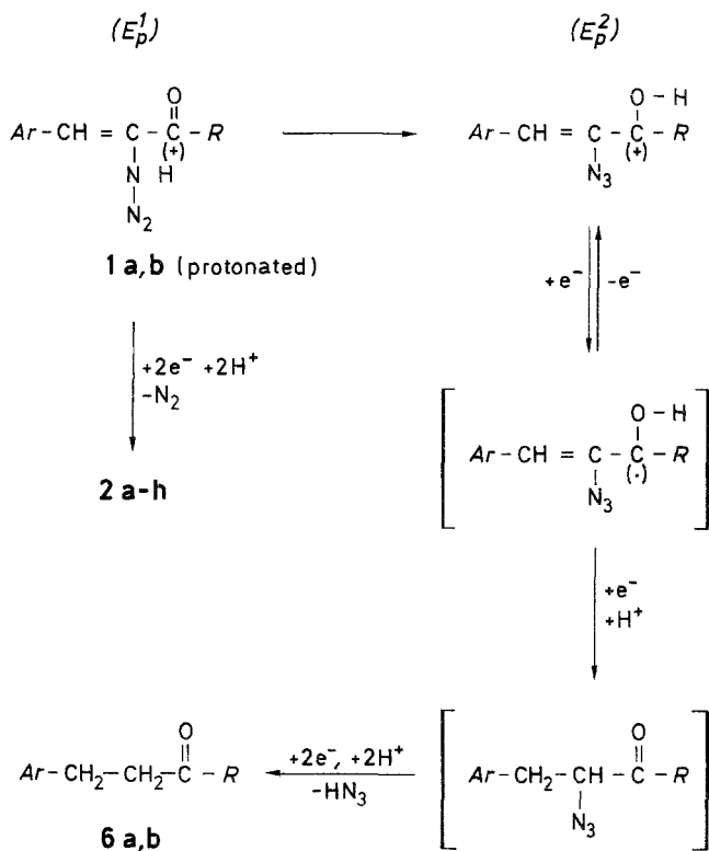
Scheme 2. Protonated forms of azidochalcones and their reduction at different potentials E_p^1 and E_p^2
