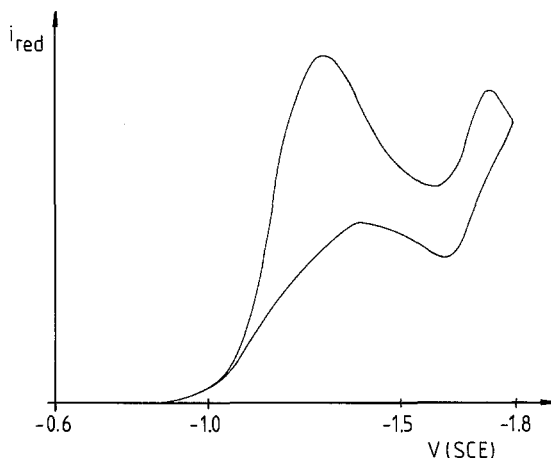
Fig. 1. CV of the reduction of azidochalcone 1b in AN/TEAB at Hg, 50 mVs -1
