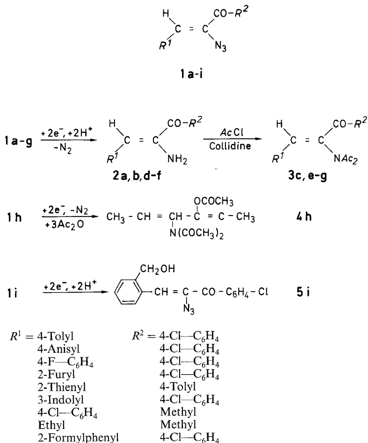
Scheme 1. Products of cathodic reduction of enazidoketones
