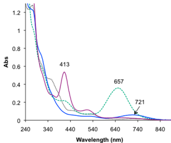
Figure 3. UV–vis spectra displaying three different products from reaction between [\text{WO}(\text{S}_2\text{C}_2\text{Ph}_2)_2]^{2-} (2) with \text{TsOH} in acetonitrile. UV–vis spectra of the reaction of 2 with 1 equiv of \text{TsOH} generating [\text{WO}(\text{S}_2\text{C}_2\text{Ph}_2)_2]^- (blue solid), the reaction of in situ generated [\text{WO}(\text{S}_2\text{C}_2\text{Ph}_2)_2]^- with additional 2 equiv of \text{TsOH} forming [\text{W}(\text{S}_2\text{C}_2\text{Ph}_2)_3] (green dashed), and the reaction of 2 with 4 equiv of \text{TsOH} generating [\text{W}(\text{MeCN})_2(\text{S}_2\text{C}_2\text{Ph}_2)_2] (4) (purple solid).
