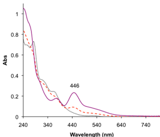
Figure 1. UV–vis spectral changes during titration of (\text{Et}_4\text{N})_2[\text{MoO}(\text{S}_2\text{C}_2\text{Ph}_2)_2] (1) (black dotted) with tosylic acid (TsOH) in acetonitrile at room temperature. An addition of 1 equiv of TsOH to 1 results in the incomplete conversion (red dashed) of 1 to [\text{Mo}(\text{MeCN})_2(\text{S}_2\text{C}_2\text{Ph}_2)_2] (3). A further addition of extra 1 equiv of TsOH leads to the complete formation of 3 (purple solid).
